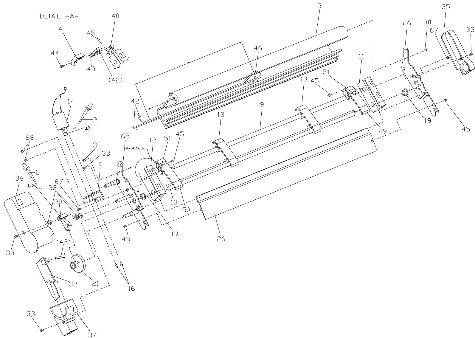
Figure 9 : LOWER TRACTOR ASSEMBLY
