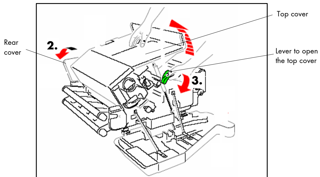
Fig.8 4.4.b Opening the rear and top cover
