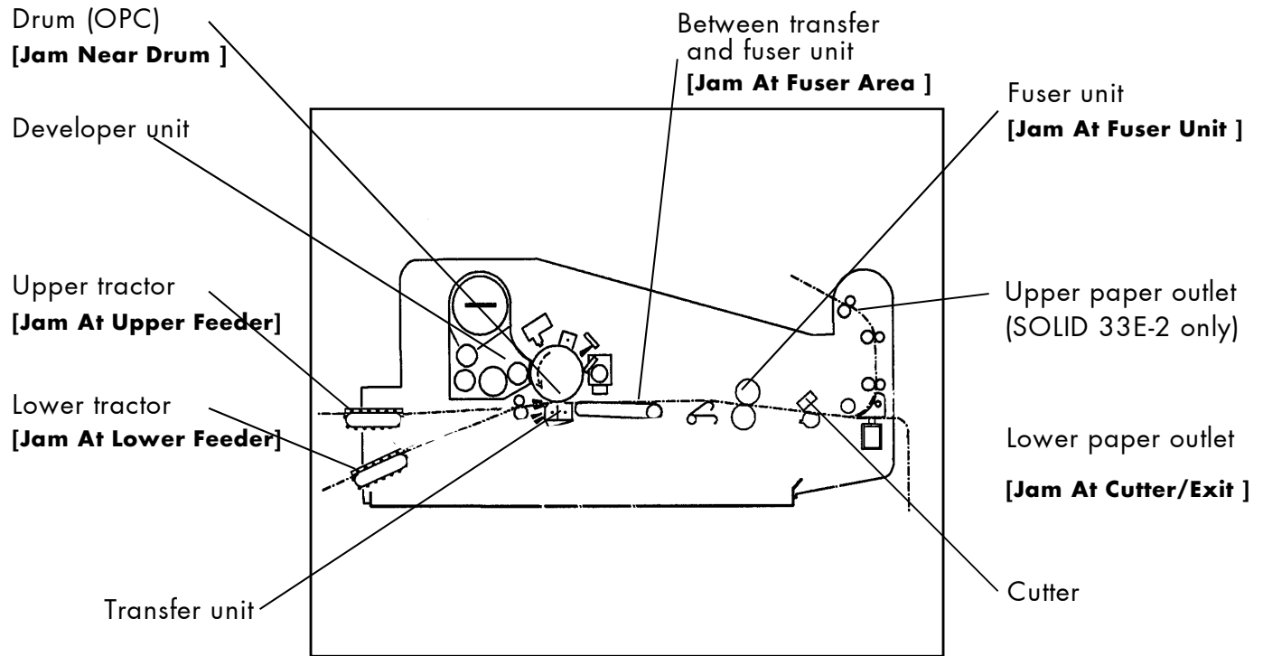
Fig. 8.4.1.a Schematic diagram of the paper paths of the SOLID 33E-2 and SOLID 58E printers incl. assignment of error messages
