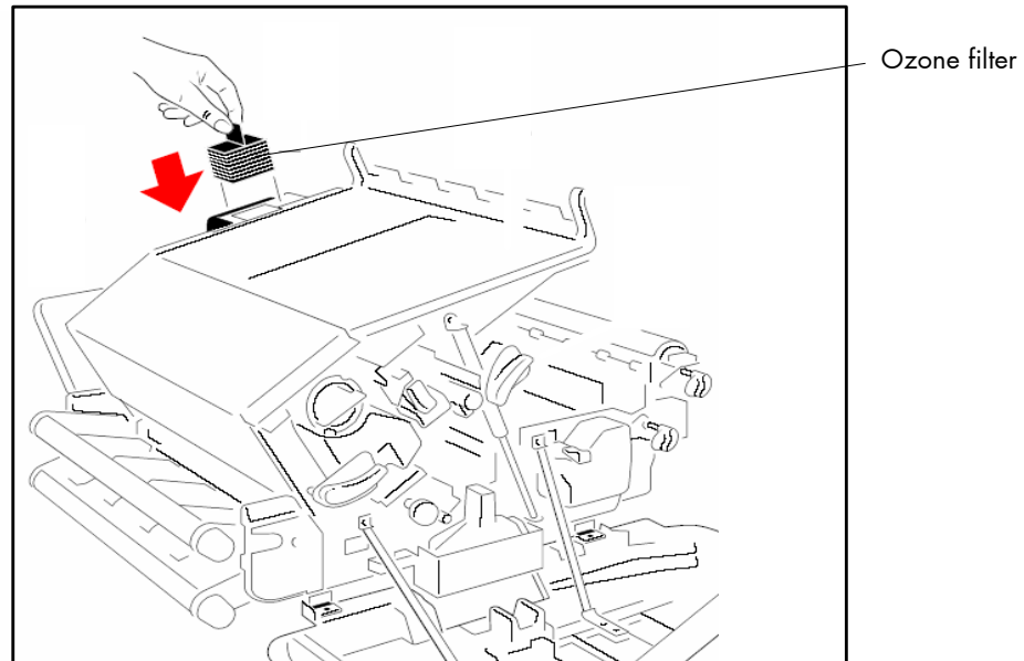
Fig. 2.4.6.a Inserting the ozone filter
