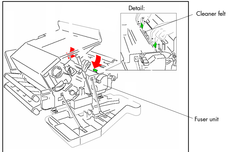
Fig. 7.1.2.f Checking the cleaner felt
