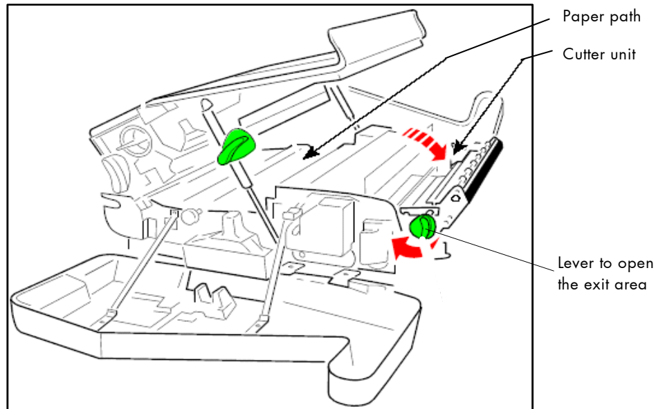
Fig. 8.4.4.c Opening the paper exit area
