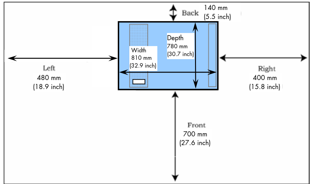
Fig. 2.3.a SOLID 33E-2 and SOLID 58E: Required space (plan view)
