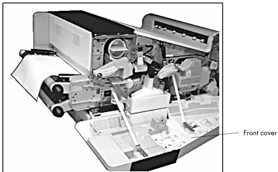
Fig. 2.4.1.a Printer opened
