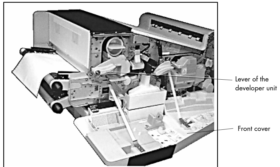
Fig. 2.4.2.a Printer opened
