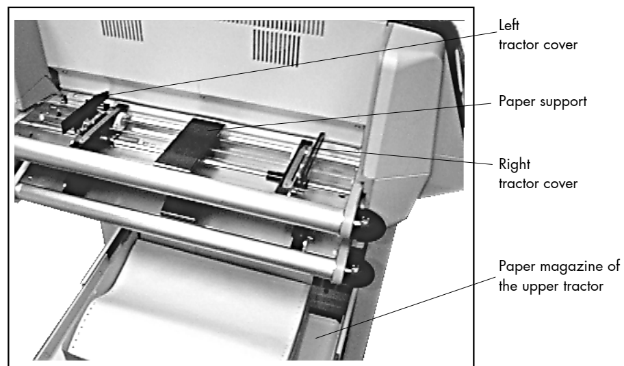
Fig. 4.1.2.b Opening the tractor covers
