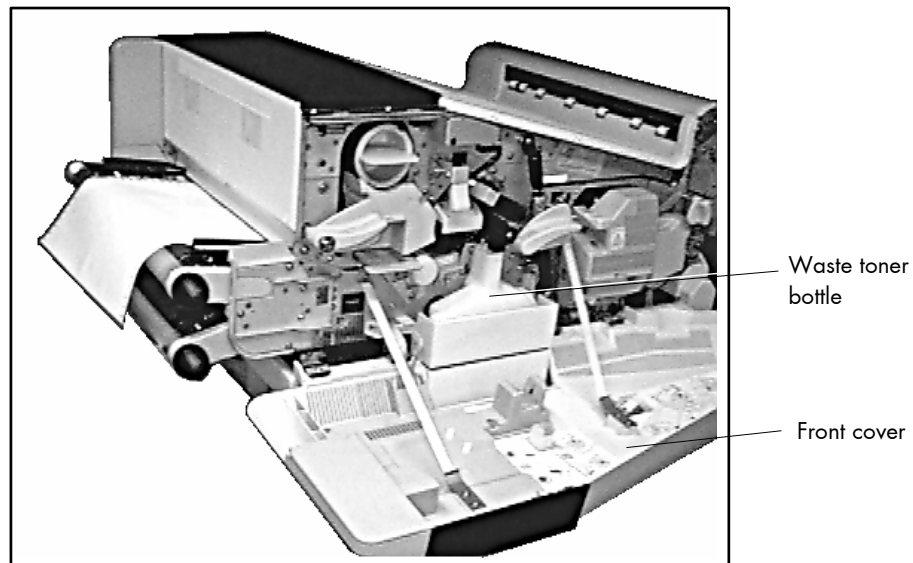
Fig. 7.1.2.a Printer opened
