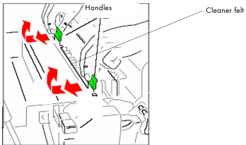
Fig. 7.4.b Removing the old cleaner felt
