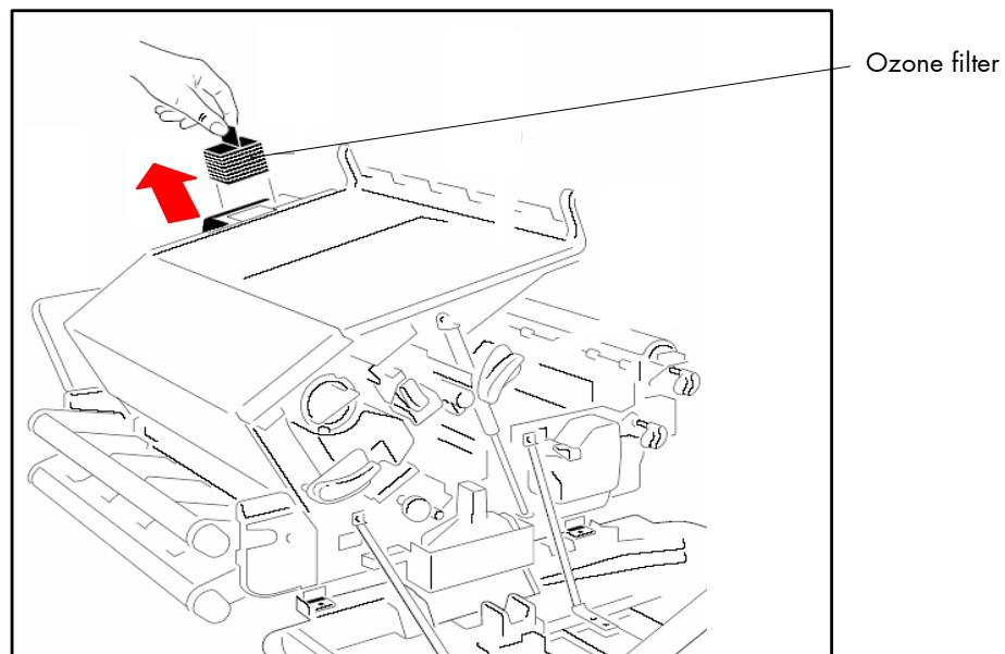
Fig. 7.5.a Removing the old ozone filter
