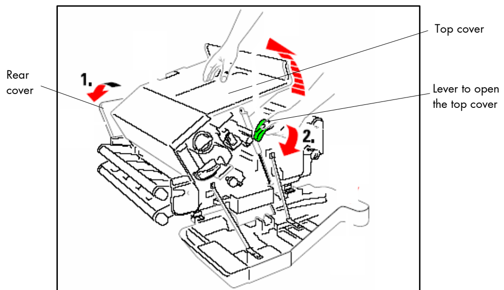
Fig. 7.4.a Opening the rear and top cover
