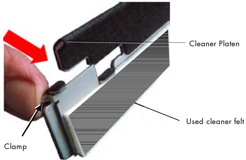
Fig. 7.4.c Removing the old cleaner felt from the cleaner platen
