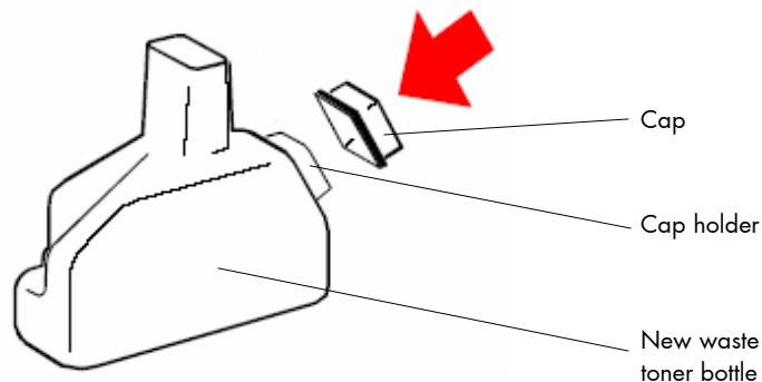
Fig. 7.3.c Preparing the new waste toner bottle
