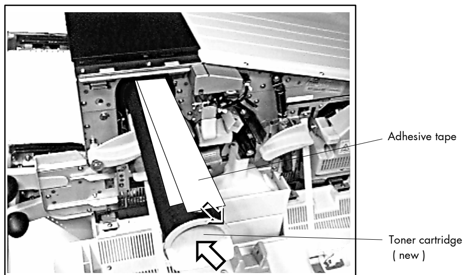
Fig. 7.2.d New toner cartridge inserting
