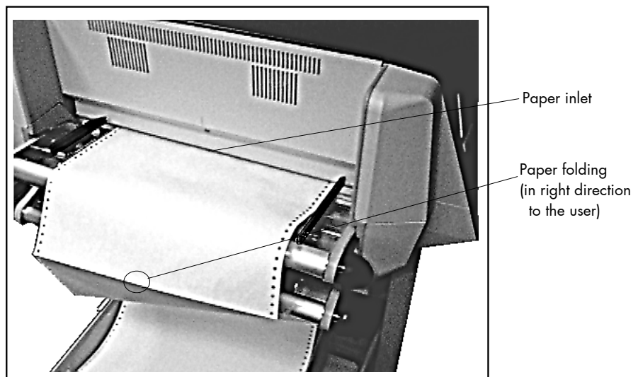
Fig. 4.1.2.d Paper inserting
