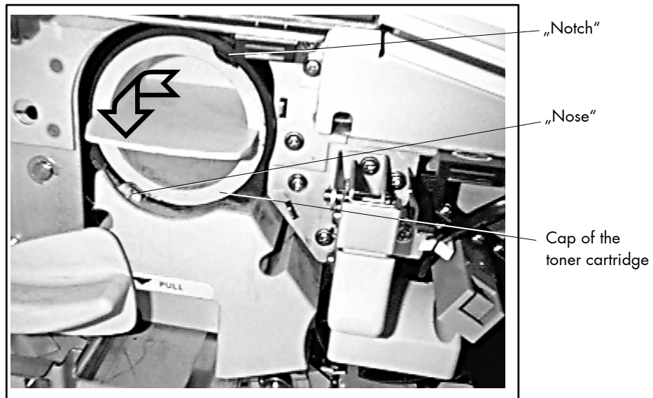
Fig. 2.4.3.e Locking the toner cartridge
