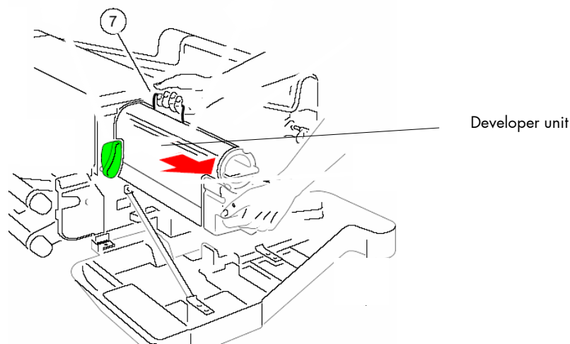
Fig. 7.1.2.c Taking out the developer unit
