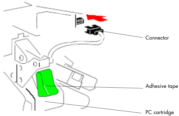
Fig. 2.4.7.b Attaching the electrical connector
