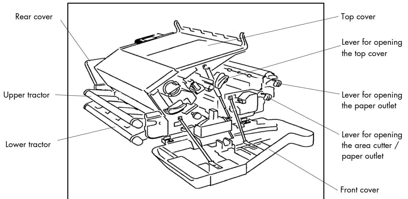
Fig. 8.4.4.d Overview: Printer SOLID 33E-2 / 58E opened
