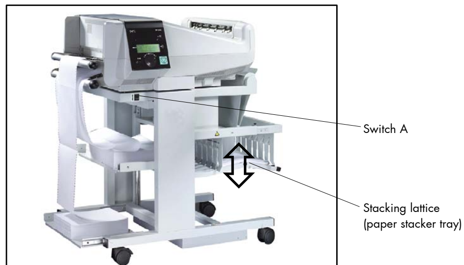
Fig. 4.2.3.2.a Driving down the stacking lattice
