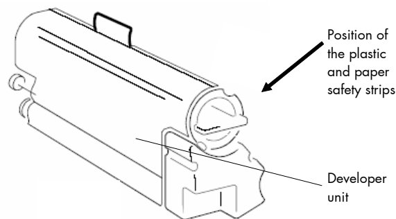
Fig. 2.4.2.d Position of the safety strips
