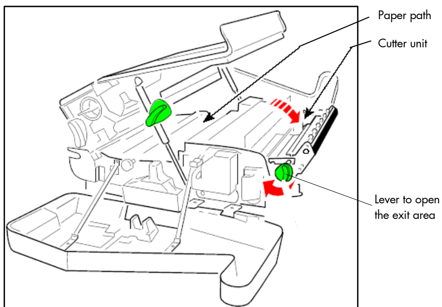
Fig. 7.1.2.e Opening the paper exit area
