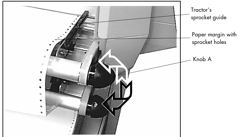
Fig. 4.1.2.c Adjusting the upper tractor to the paper width
