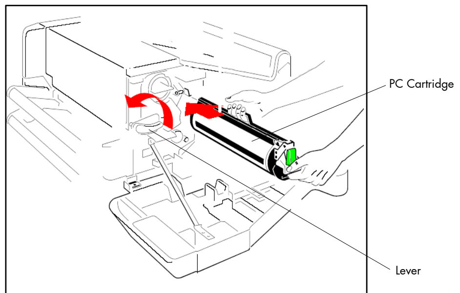
Fig. 2.4.7.a Unlocking the developer unit and inserting the PC cartridge
