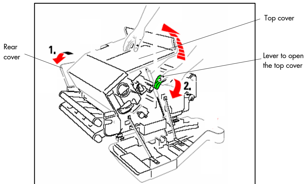
Fig. 7.1.2.d Opening the rear and top cover
