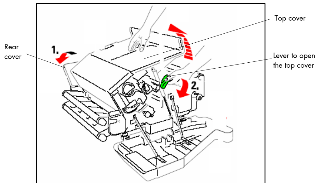
Fig. 7.3.a Opening the rear and top cover
