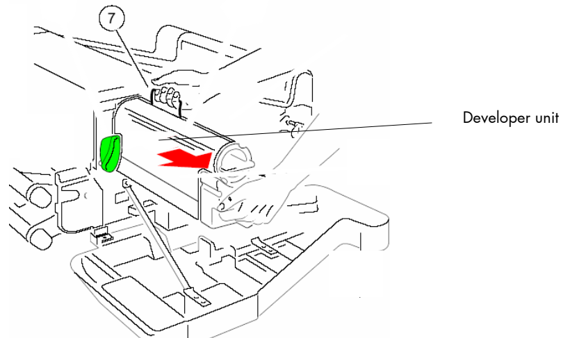
Fig. 2.4.2.c Taking out the developer unit
