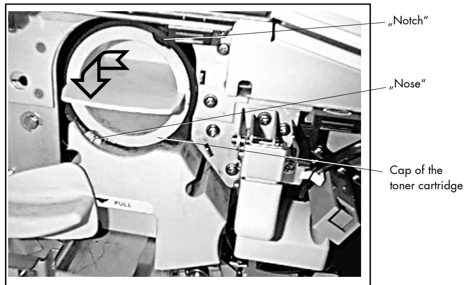
Fig. 7.2.e Locking the toner cartridge
