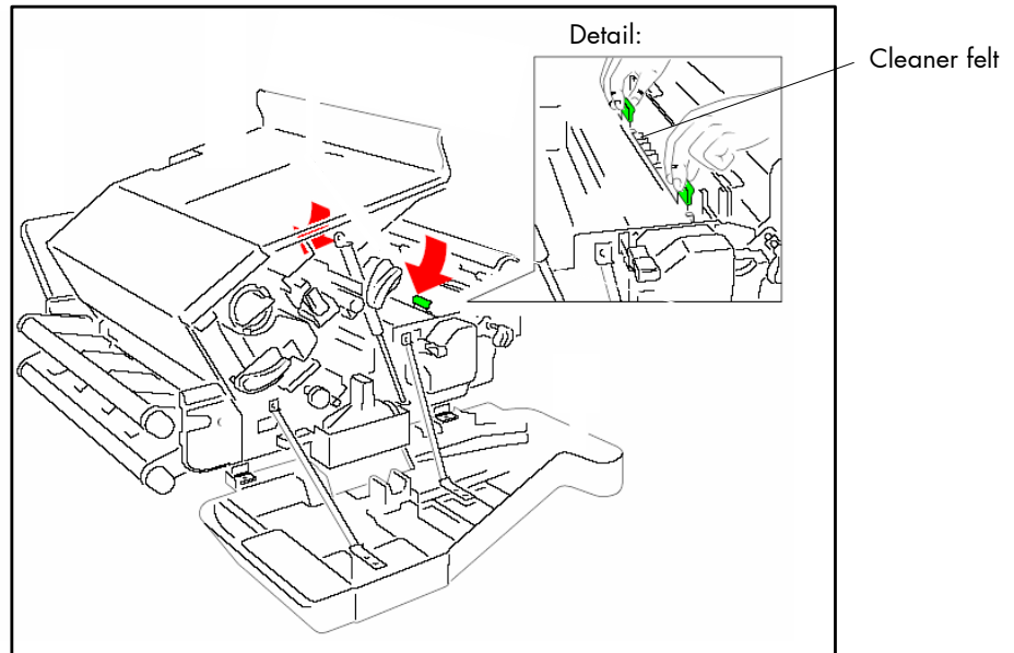
Fig. 2.4.5.a Inserting the cleaner felt
