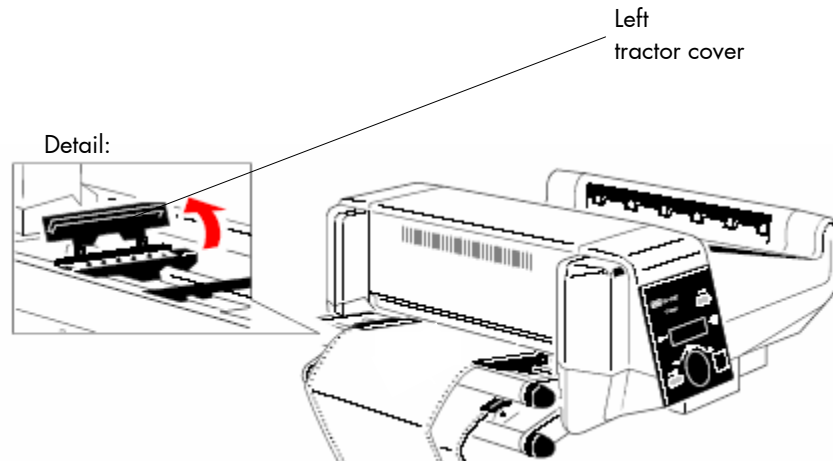
Fig. 8.4.3.a Opening the tractor covers
