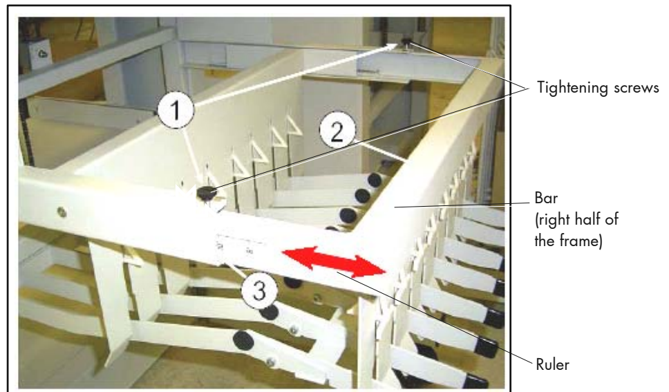
Fig. 4.2.3.1.a Adjusting the paper stacker system to the paper size
