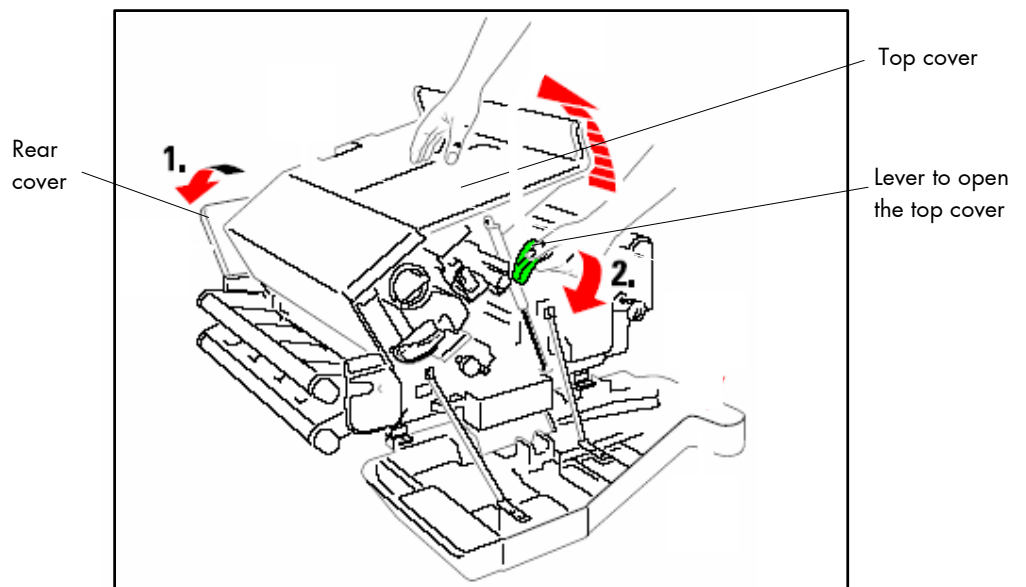
Fig. 2.4.4.a Opening the rear and top cover
