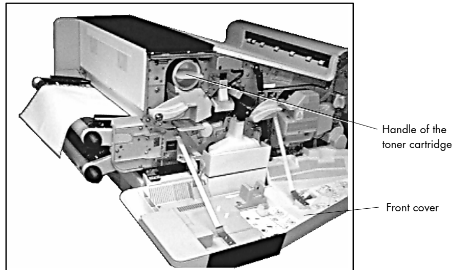
Fig. 7.2.a Printer's front cover open
