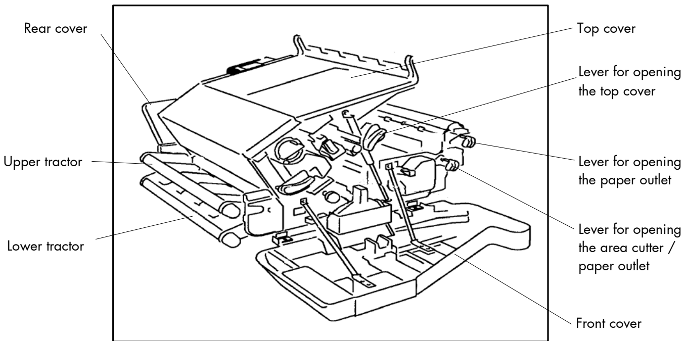
Fig. 2.2.d Printer SOLID 33E-2 / 58E opened
