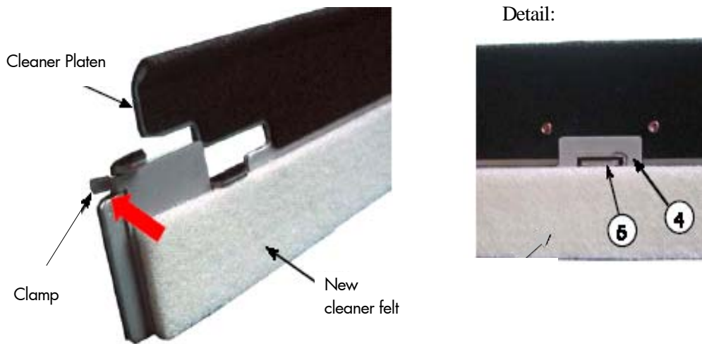
Fig. 7.4.d Mounting the new cleaner felt to the cleaner platen
