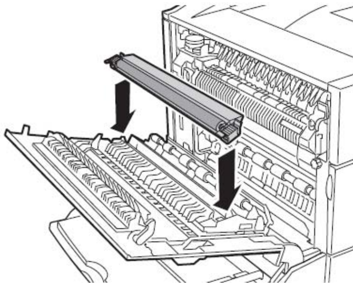
Fig. 6.2.f Sliding the new transfer roller into place
